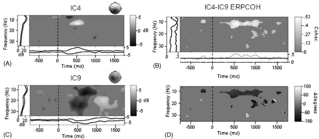
Fig. 6. Time/frequency decompositions of independent component activities. Time/frequency decomposition was applied to the activities of two independent EEG components using sinusoidal wavelet transforms, 3 cycles in length at the lowest frequency (6 Hz), increasing linearly with frequency up to nine cycles at the highest plotted frequency (35 Hz). Using this approach, it is possible to obtain reasonable time and frequency stability at all frequencies. (A–B) Event-related spectral perturbation (ERSP) plots showing mean changes in spectral power during the epoch, relative to a 1-s pre-stimulus baseline (plotted vertically on the left). Component IC4 shows a transient increase near 12 Hz centered at 500 ms, while component IC9 shows a power decrease in this range following 500 ms. (C–D) Phase cross-coherence (ERPCOH) magnitude and phase delay between the two components shown in panels A–B, zero-masked in regions in which cross-coherence magnitude was not significant ( P > 0.01 ). The components appear to become partially synchronized above 10 Hz (coherence \leq 0.53 ) during the period 400–1000 ms with a phase offset near -120^\circ . Under the minimum phase assumption, this implies that high-alpha activity of IC9 tends to lead that of IC4 during this period by about 30 ms.
