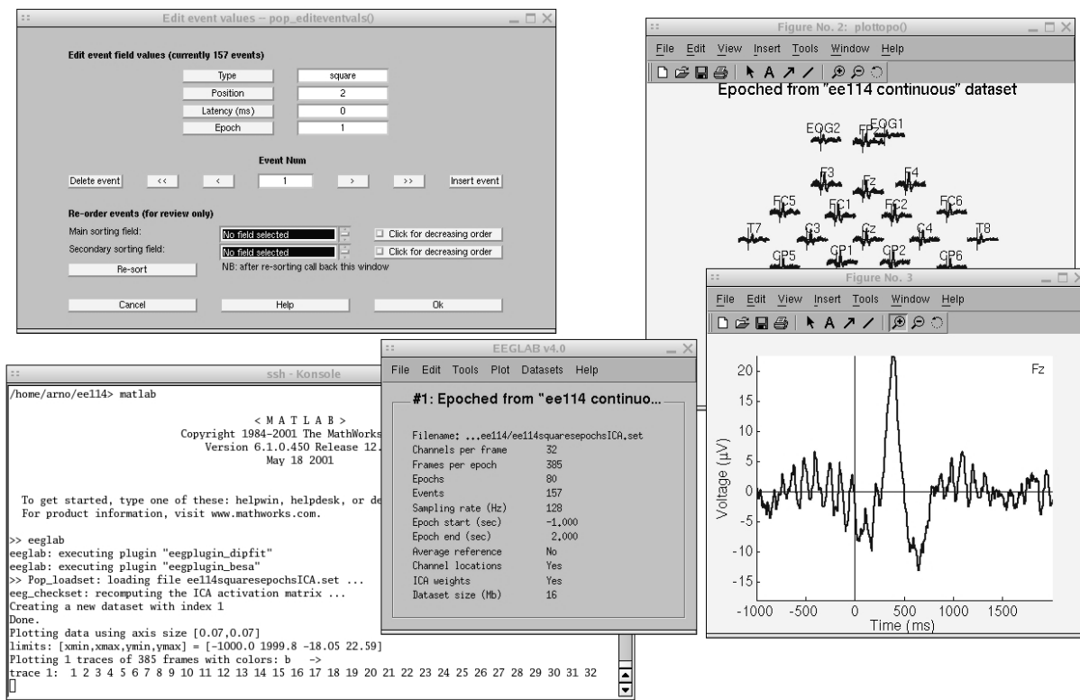
FIG. 1. Sample EEGLAB session. Screen capture of an EEGLAB user session running under Linux. Users call EEGLAB functions from the main window menus (center). Warnings and data processing messages are shown in the Matlab command line window (lower left), which can also be used to call EEGLAB or other data processing functions directly.
